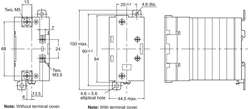
Mounting Holes
