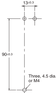
Mounting Holes
