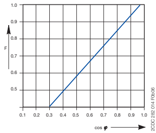
Derating curve
