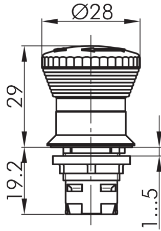
Dimensional drawing:
