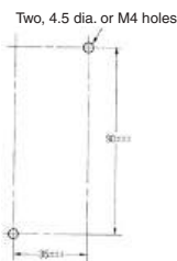
Mounting Holes
