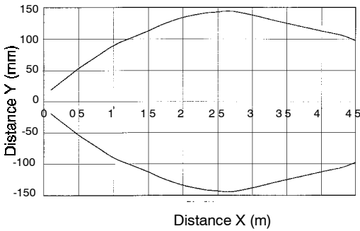
E3F2-7□□-4□ (Through-beam)
