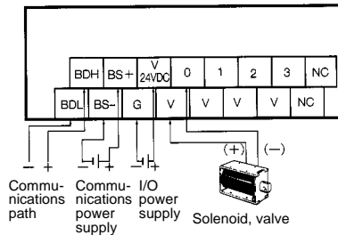
SRT1-OD04, SRT2-OD04
