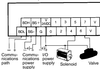
SRT1-OD08, SRT2-OD08
