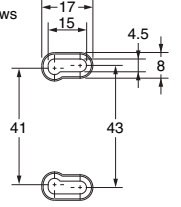
Mounting Holes (Enlargement)
